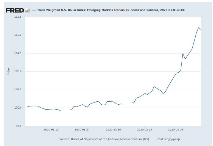
FIGURE 3: TRADE WEIGHTED U.S. DOLLAR INDEX: EMERGING MARKET ECONOMIES, GOODS AND SERVICES, 2020-01-01=100
